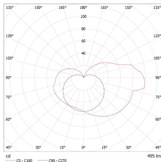
Lucis S5.L12.A350.0W ASTERION LED / LDC (Polar)
